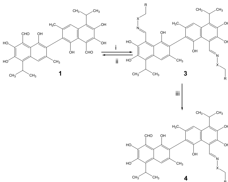
Scheme 1. Reagents and conditions: (i) \text{RCH}_2\text{XNH}_2 , DCM, IPA; (ii) \text{AcOH} , \text{Et}_2\text{O} , \text{H}_2\text{SO}_4 , 0^\circ\text{C} , 16 h; (iii) \text{AcOH} , \text{Et}_2\text{O} , \text{H}_2\text{SO}_4 , 0^\circ\text{C} , 4 h.
