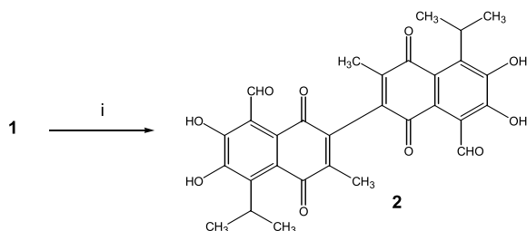
Scheme 2. Reagents and conditions: (i) FeCl 3 , acetone, AcOH, 100 °C, 2 h, then ether, 20% aq H 2 SO 4 .
